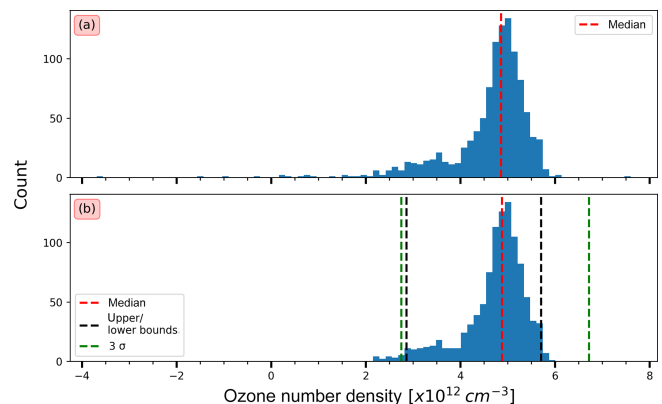
Figure 12. As in Fig. 10 but for ozone data at 20 km between 65 and 75° S in December.
