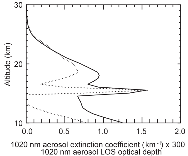
Figure 6. Single profile of 1020 nm aerosol extinction coefficient \times 300 (dashed line), along with the computed LOS optical depth (solid line). The extinction coefficient, particularly below the cloud located near 15 km, is clearly not representative of the impact of aerosol on ozone determinations at that altitude.
