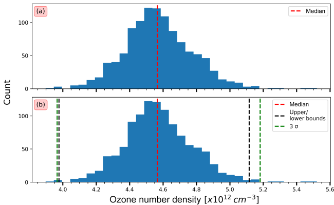
Figure 10. Probability density function of SAGE II ozone at 25 km between 25 and 35° S for July. (a) Probability density function of SAGE II ozone before any screening is applied to the data. (b) Probability density function of SAGE II ozone after the 200 % uncertainty rule and the aerosol LOS optical depth rule were applied. The red line indicates the median of the distribution shown in each panel, while the dashed black lines represent the upper and lower boundaries calculated as described in the text. As a reference, panel (b) includes 3 times the standard deviation of the distribution ( 3\sigma ) to represent the selection criteria similar to current rule no. 11. All data points that lie outside the dashed black lines will be removed from the data set. For more details, see the main text.
