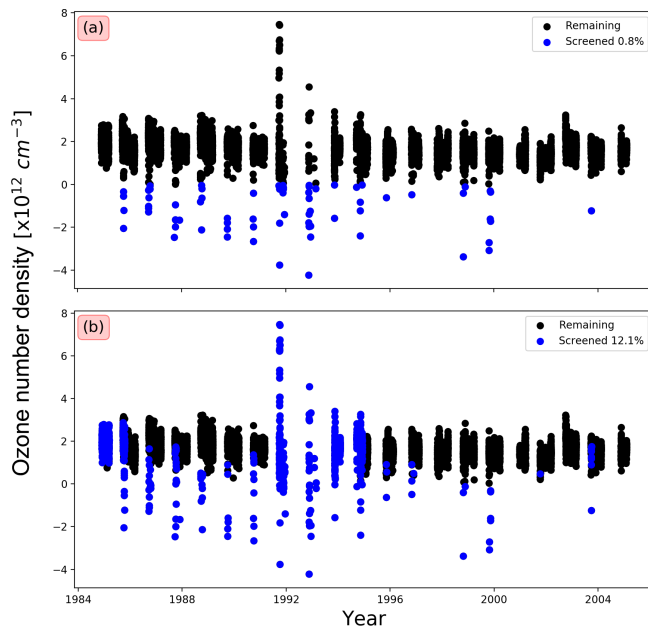
Figure 9. Ozone number density at 12 km between 65 and 75° S: when (a) SAGE II ozone data at the given latitude bin and altitude that remain (black dots) after ozone values with a relative error of 200 % are removed (blue dots), and when (b) SAGE II ozone data at the given latitude bin and altitude that remain (black dots) after ozone values where the aerosol LOS optical depth exceeds 2 are removed (blue dots).
