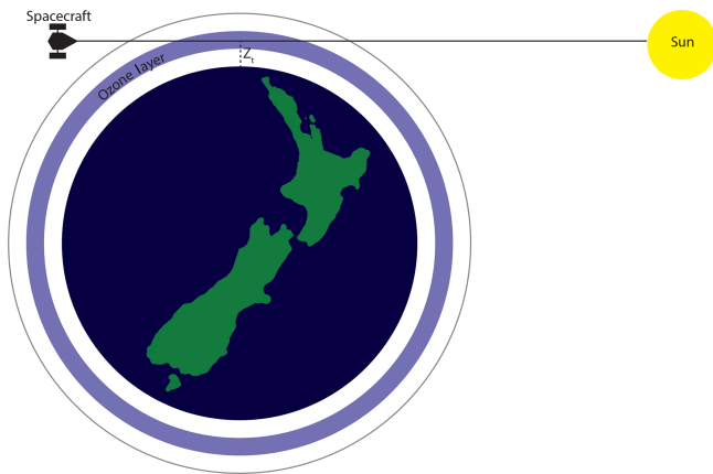
Figure 1. A schematic diagram showing the solar occultation viewing geometry that is exploited by SAGE II to make measurements of atmospheric constituents. Z_t denotes the tangent altitude. For more details, see the main text.
