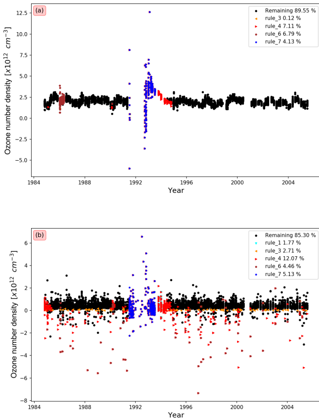
Figure 3. SAGE II ozone number density at 20 km between 5° S and 5° N (a) and 16.5 km between 25 and 15° S (b) before and after data usage rules (Sect. 3) have been applied, as indicated in the legend. Each rule is associated with a percentage of data points that will be removed from the data sets if the rule is applied. For more details, see the main text.
