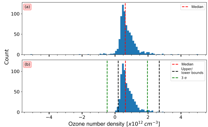
Figure 11. As in Fig. 10 but for ozone data at 18 km between 15 and 25° N for January.
