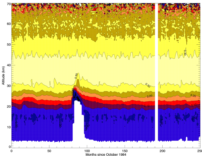
Figure 5. Measurement fraction, f , for 5^\circ N for all SAGE II data (no clearing) for the entire lifetime of the instrument. Note that the Mount Pinatubo period, particularly from month 81 (June 1991) to through to roughly month 100 (the end of 1992), shows a clear reduction of the value of f above 18 km to as high as 35 km. Though several other volcanic events occur during the SAGE II lifetime (e.g. Nevado del Ruiz and Nyamuragira), none of these are readily apparent in f since they were an order of magnitude or more smaller than the Mount Pinatubo event.
