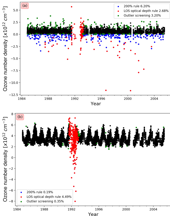
Figure 13. Ozone number density at 17 km between 15 and 25° N (a) and at 20.5 km between 25 and 35° S. The black dots represent the full SAGE II ozone data sets at the given altitude and latitude band, while the coloured dots represent the ozone values that would be removed by applying the new rules (as indicated in the legend). Note that all rules were applied individually to all data points.
