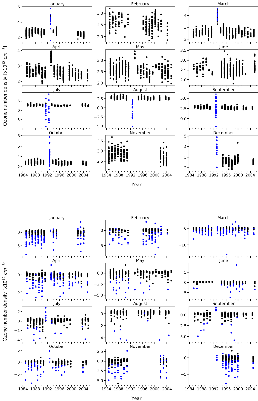
Figure 8. Remaining SAGE II ozone at 21 km (top) and 16 km (bottom) between 5^{\circ} and 15^{\circ} S for each month of all years (black) after the LOS optical depth rule has been applied to the ozone data set (blue dots).
