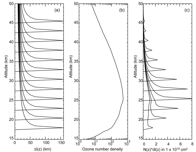
Figure 4. (a) Profiles of \Delta l_{i,j} (in km) for tangent altitudes from 18 to 45.5 km in 2.5 km steps in tangent altitude, (b) a representative ozone profile n_{\text{O}_3}(z) in \text{cm}^{-3} , and (c) the product of the curves in (a) with the ozone profile shown in (b) so that \Delta l_{i,j} \times n_{\text{O}_3}(z) in 1 \times 10^{19} \text{ cm}^{-2} . The profiles were taken from the November 1984 v7.00 data set, event no. 1.
