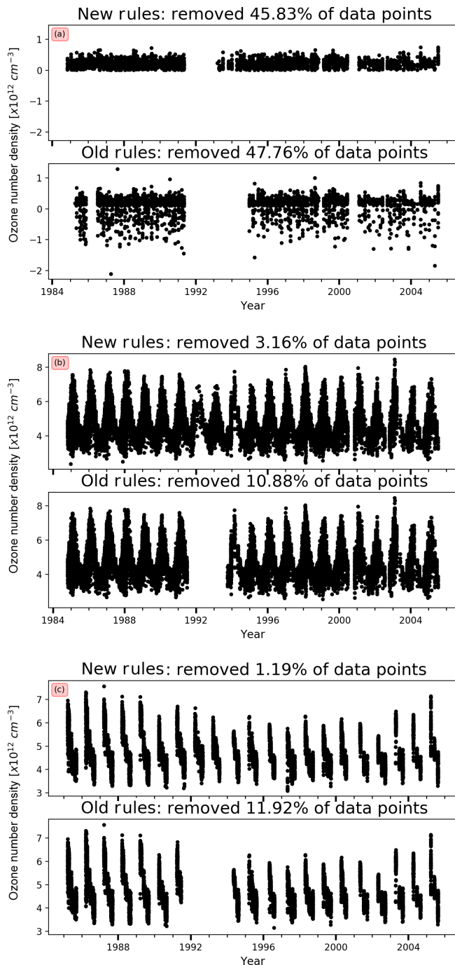
Figure 14. SAGE II ozone at (a) 16 km between 5° S and 5° N, (b) 20 km between 45 and 55° N, and (c) 20.5 km between 65 and 75° N. SAGE II data shown represent the remaining ozone data after the new (top) and current (bottom) rules were applied.
