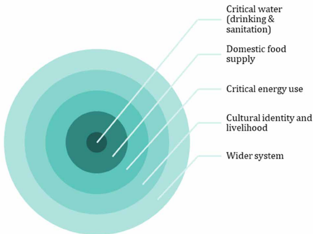
Figure 2: Ordering possible channels for drought to impact human health and wellbeing
