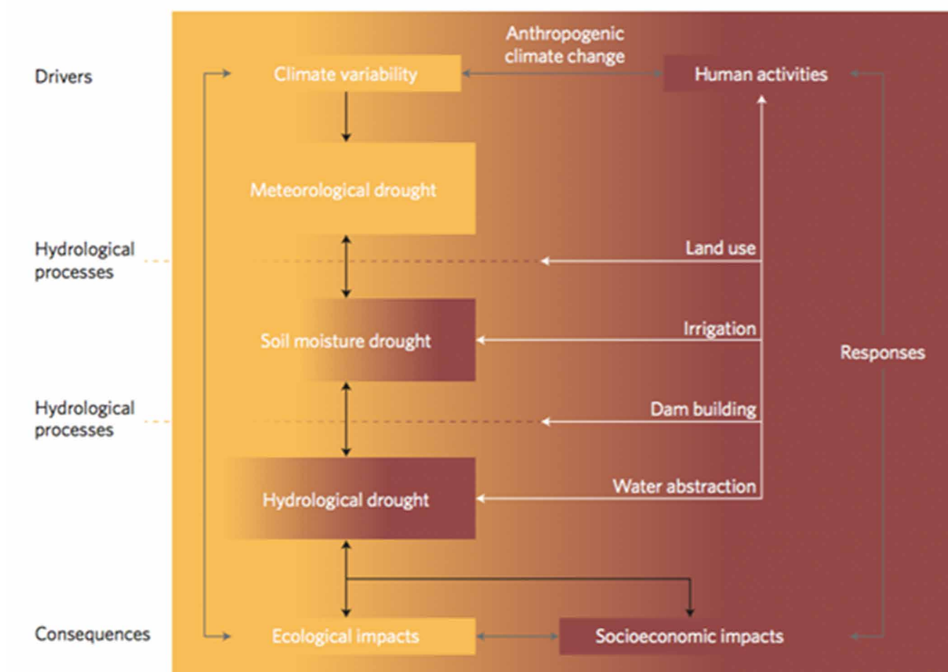
Figure 1: Drought system (Van Loon et al., 2016)
