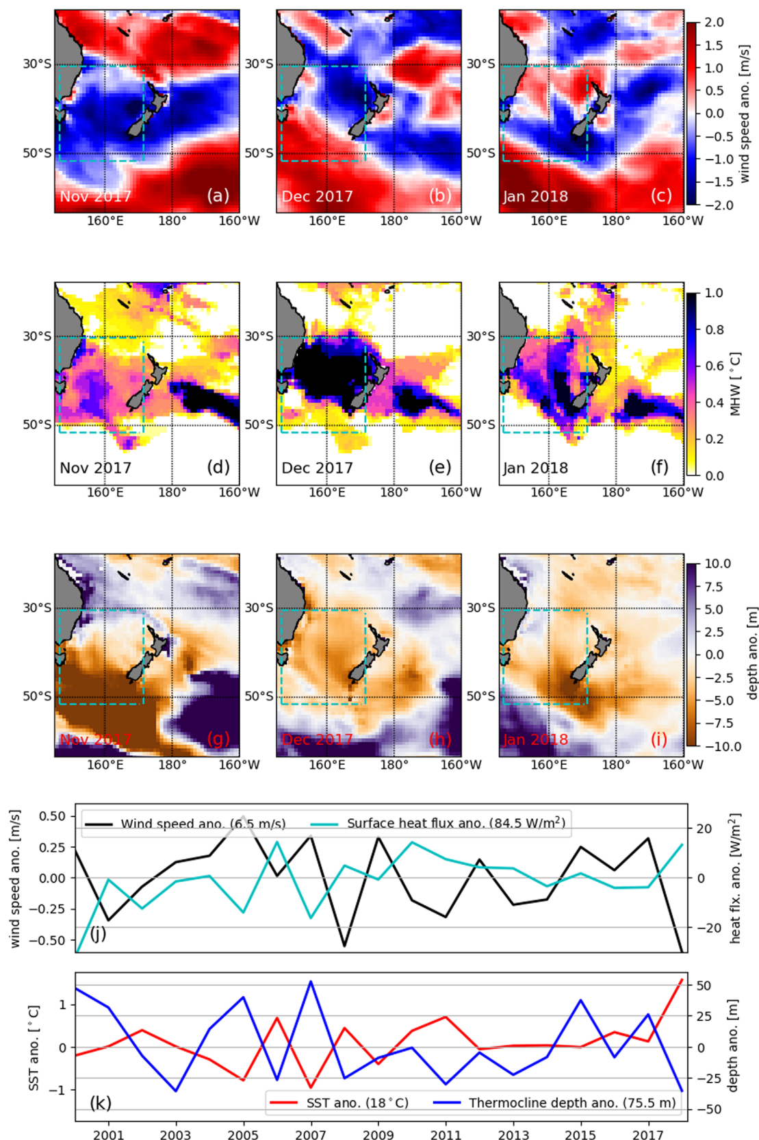
Figure 3. Ocean modelling: driving mechanisms for the MHW. Monthly mean values for wind speed anomaly (a)–(c), MHW intensity (d)–(f), and mixed layer depths anomaly (g)–(i) for the period November 2017–January 2018 based on the model hindcast. To identify MHWs the Hobday et al. (2016) definition has been used. The light blue dashed box identifies the region which has been used to compute area-averages for timeseries in (j) and (k). Annual NDJ (Nov–Dec–Jan) area averaged (Tasman box) anomalies for surface heat fluxes ( \text{W m}^{-2} ) and wind speeds ( \text{m s}^{-1} ) are presented in (j) and SST ( ^{\circ}\text{C} ) and thermocline depth (m) in (k). Mean climatological values for NDJ are given in parentheses.
