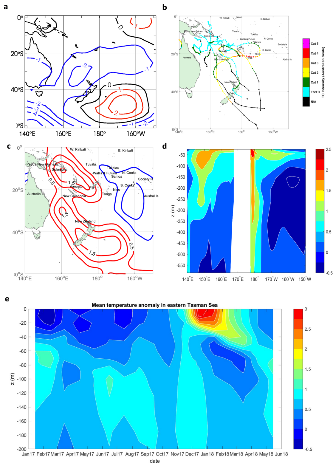
Figure 2. Atmospheric pressure anomalies, tropical cyclone occurrence and sub-surface temperature anomalies. (a) NCEP December 2017–February 2018 mean sea level pressure anomalies using the 1981–2010 reference period, contour interval 1hPa, negative contours blue, positive red and zero is black; (b) Named tropical cyclone (TC) tracks for the southwest Pacific for the 2017/18 austral summer to the end of April 2018 based on the latest SPEArTC dataset (Diamond et al 2012); (c) TC frequency of occurrence anomalies (right panel) calculated as the differences from the 1981–2010 climatology from SPEArTC from those TC seasons, contour interval is 0.5 TC occurrences; red contours positive; blue contours negative; zero contour omitted; (d) December 2017–February 2018 sub-surface temperature anomalies for the Pacific Ocean from 40–45°S using the 1981–2010 reference period for Global Ocean Data Assimilation System (GODAS) sub-surface temperatures; (e) regionally-averaged ARGO float measurements for the eastern Tasman Sea (35–45°S, 160–172.5°E) of the mean temperature anomaly over the period January 2017–May 2018.
