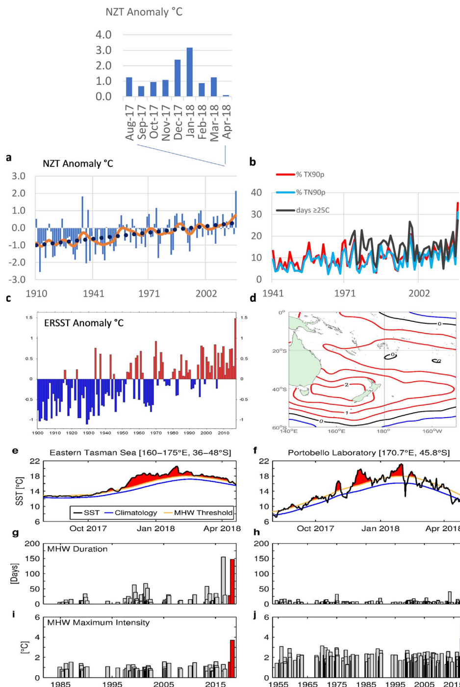
Figure 1. The 2017/18 New Zealand atmosphere and ocean heatwaves. (a) The New Zealand air temperature (NZT) series 1909–2018 summer (DJF) anomaly compared with the 1981–2010 normal. The red curve is a 15 year filtered average, and black dotted line the trend. Inset: Mean NZT August 2017–April 2018 anomalies. (b) Summer (DJF) indices of climate extremes for New Zealand from station data and VCSN. Station indices are warm days in red (percentage of time when daily maximum temperature > 90th percentile), warm nights in blue (percentage of time when daily minimum temperature > 90th percentile). The VCSN summer (DJF) count when daily maximum temperature \geq 25^{\circ}\text{C} (in black). (c) Summer (DJF) SST anomalies 1900–2018 (ERSSTv5) averaged over the Tasman Sea region ( 26^{\circ}\text{S} – 46^{\circ}\text{S} , 150^{\circ}\text{E} – 174^{\circ}\text{E} ) using 1961–1990 climatology (Bureau of Meteorology, Australia). (d) Composite December 2017–January 2018 SST anomalies (from NOAA ERSSTv5) using the 1981–2010 normal with contours at 0.5^{\circ}\text{C} intervals. (e)–(j). First row: time series of summer (Dec–Feb) sea surface temperature (SST) climatology (1981–2011; blue), 90th percentile MHW threshold (orange) and summer 2017/18 SST time series (black) from (e) the eastern Tasman Sea ( 160 – 175^{\circ}\text{E} , 36 – 48^{\circ}\text{S} ) and (f) the Portobello Marine Laboratory ( 45.88^{\circ}\text{S} , 170.50^{\circ}\text{E} ). The red shaded regions identify periods associated with MHWs detected in the SST time series from each location using the Hobday et al (2016) definition. Second row: the duration of each MHW detected in the SST time series for (g) the eastern Tasman Sea and (h) Portobello Marine Laboratory. The red shaded bar highlights MHWs detected during summer 2017/18. Third row: as above but showing the maximum intensity of each MHW detected in the SST time series for (i) the eastern Tasman Sea and (j) Portobello Marine Laboratory.
