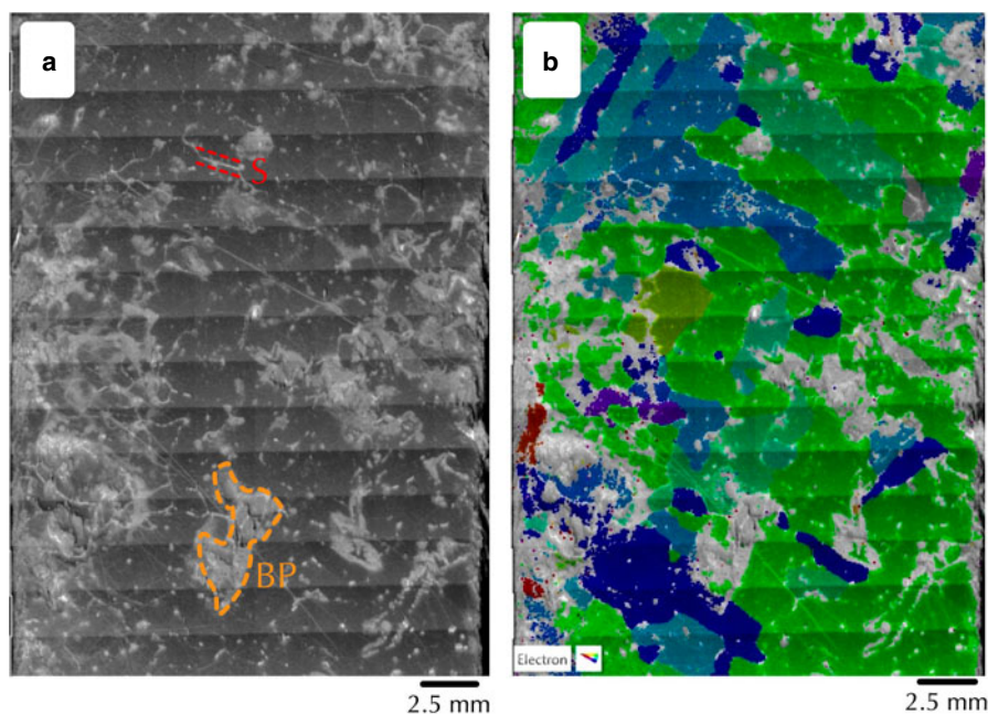
Fig. 4. Some issues for EBSD on sea ice. (a) Secondary electron image montage of CI-h from the SEM shows salt (bright flecks on grain boundaries: S) which was expelled along grain boundaries and exposed brine pockets (grey holes: BP). (b) Image to show level of indexing in raw EBSD data. Coloured pixels have a good quality EBSD solution. Non-indexed pixels are transparent so that the underlying greyscale image (as in Fig. 4a) is visible.
