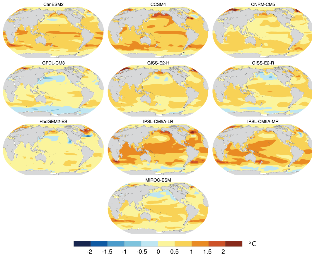
Figure 12. Estimated sea surface temperature response pattern (°C) to anthropogenic forcing, calculated from 10 different CMIP5 models (as labelled). The temperature responses are calculated for each month (January–December) but are shown here as annual averages.
