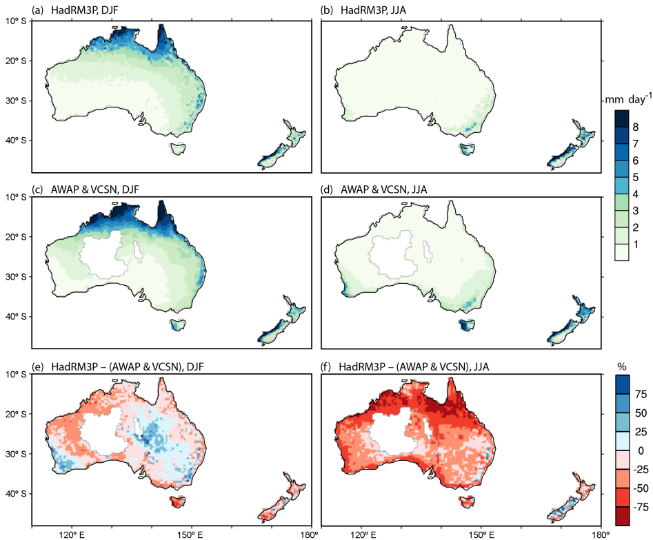
Figure 4. As in Fig. 2 but showing seasonal average precipitation ( \text{mm day}^{-1} ). The difference fields are expressed as percentages relative to the observational datasets.
