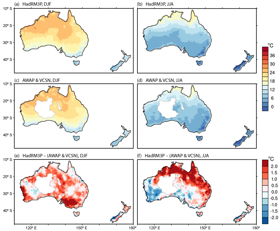
Figure 3. As in Fig. 2 but showing seasonal average minimum temperature ( ^{\circ}\text{C} ).
