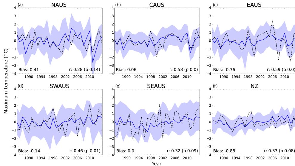
Figure 5. Time series of summertime (December–February) average maximum temperature for the respective study regions (as labelled) for 1986–2014. Ensemble-mean values from weather@home simulations are shown by the solid line (5–95th percentile shaded envelope) while the observations (AWAP over Australia and VCSN over New Zealand) are shown by the dashed line. The time series are given as anomalies relative to the mean of the entire period. The bias between the medians for the model and observations is indicated, along with the Pearson correlation coefficient ( r ; calculated using a two-sided test) and p value for testing non-correlation.
