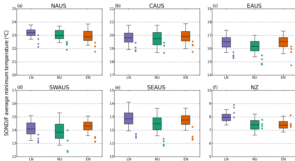
Figure 9. As in Fig. 8 but showing minimum temperature.
