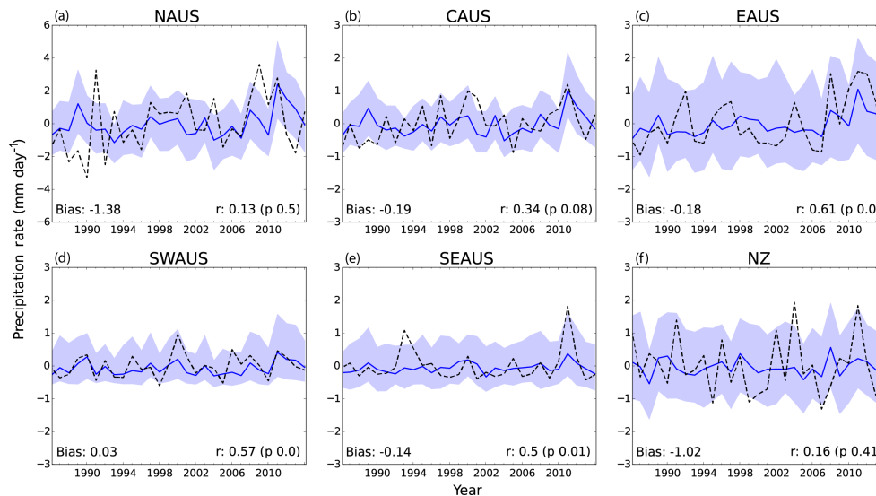
Figure 7. As in Fig. 5 but showing average precipitation.
