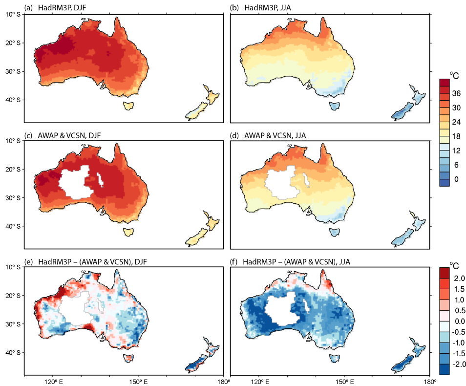
Figure 2. Seasonal average daily maximum temperatures ( ^{\circ}\text{C} ) for 1985–2014 for DJF (left), and JJA (right), from the weather@home regional model HadRM3P (top), and the observational datasets (middle; AWAP over Australia and VCSN over New Zealand). The bottom panels show the difference between HadRM3P and the corresponding observational dataset.
