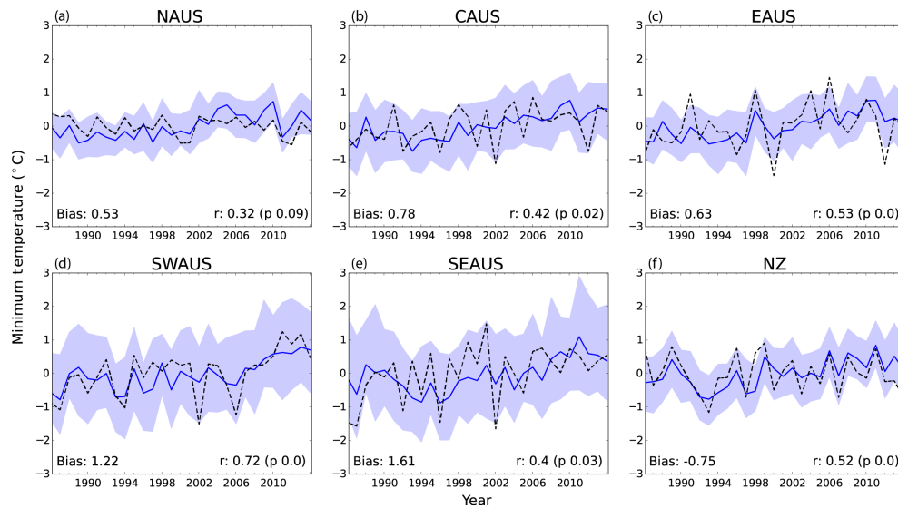
Figure 6. As in Fig. 5 but showing average minimum temperature.
