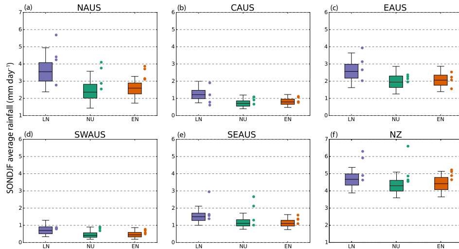
Figure 10. As in Fig. 8 but showing precipitation.
