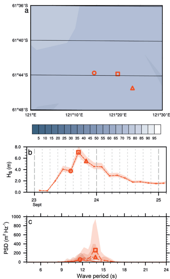
Fig. 13. (a) The location of the WIOS (markers) on 23 September 2012 at 14:00, 17:00 and 20:00 with ice concentration (%) contours. (b) The significant wave heights, H_s , over time. (c) The PSD on 23 September 2012 at 14:00, 17:00 and 20:00. The circle, square and triangle markers correspond to the 23 September 2012 at 14:00, 17:00 and 20:00, respectively. The shaded regions in (b) and (c) give the 90% confidence intervals.
