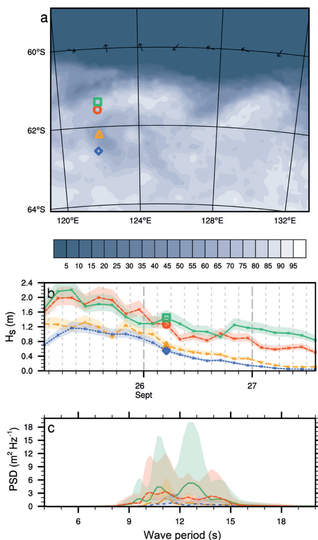
Fig. 9. Same as Figure 8, but for data from 26 September 2012 at 05:00.
