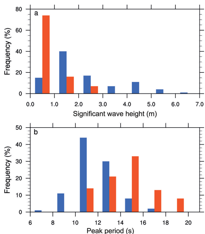
Fig. 7. The distribution of (a) significant wave heights and (b) the peak periods for the full dataset. The blue and red bars represent data when the WIIOS are within and beyond 100 km of the ice edge, respectively.
